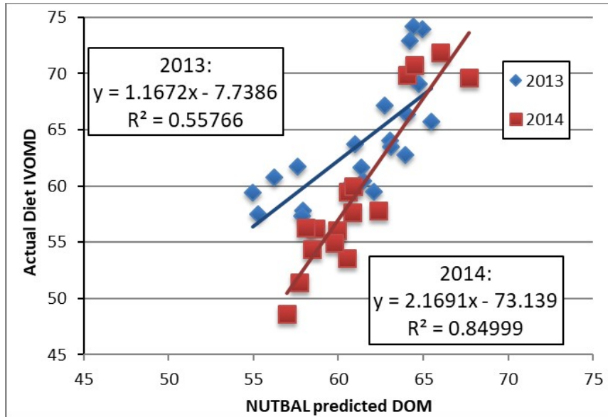
Figure 2. Regression of actual dietary in vitro organic matter digestibility (IVOMD) on fecal NIRS prediction of dietary digestible organic matter (DOM) to validate ability of fecal NIRS to predict actual dietary IVOMD. Regression relationships differed among years ( P < 0.05 ). Coefficient of variation ( r^2 ) estimates proportion of variation in actual values explained by predicted values. R^2 values range from 0 to 1 with those closer to 1 being better. The regression intercept should be 0 and slope should be 1 for a 1:1 relationship between predicted and actual values. Intercept and slope were similar to 0 and 1 ( P > 0.05 ), respectively, in 2013, but differed from 0 and 1 ( P < 0.05 ) in 2014.
