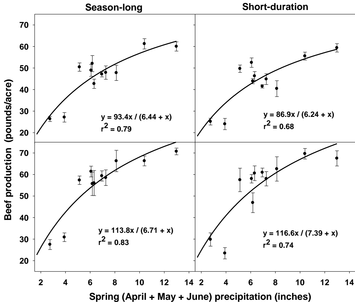
Figure 3. Hyperbolic relationships between beef production (pounds/acre, mean \pm 1 standard error) and spring (April+May+June) precipitation (inches) for season-long and short-duration rotational grazing at moderate (top panels) and heavy (bottom panels) stocking rates on northern mixed-grass prairie at the USDA-Agricultural Research Service, High Plains Grasslands Research Station near Cheyenne, WY, USA for the 1991-2006 study years (modified from Derner et al. 2008).
